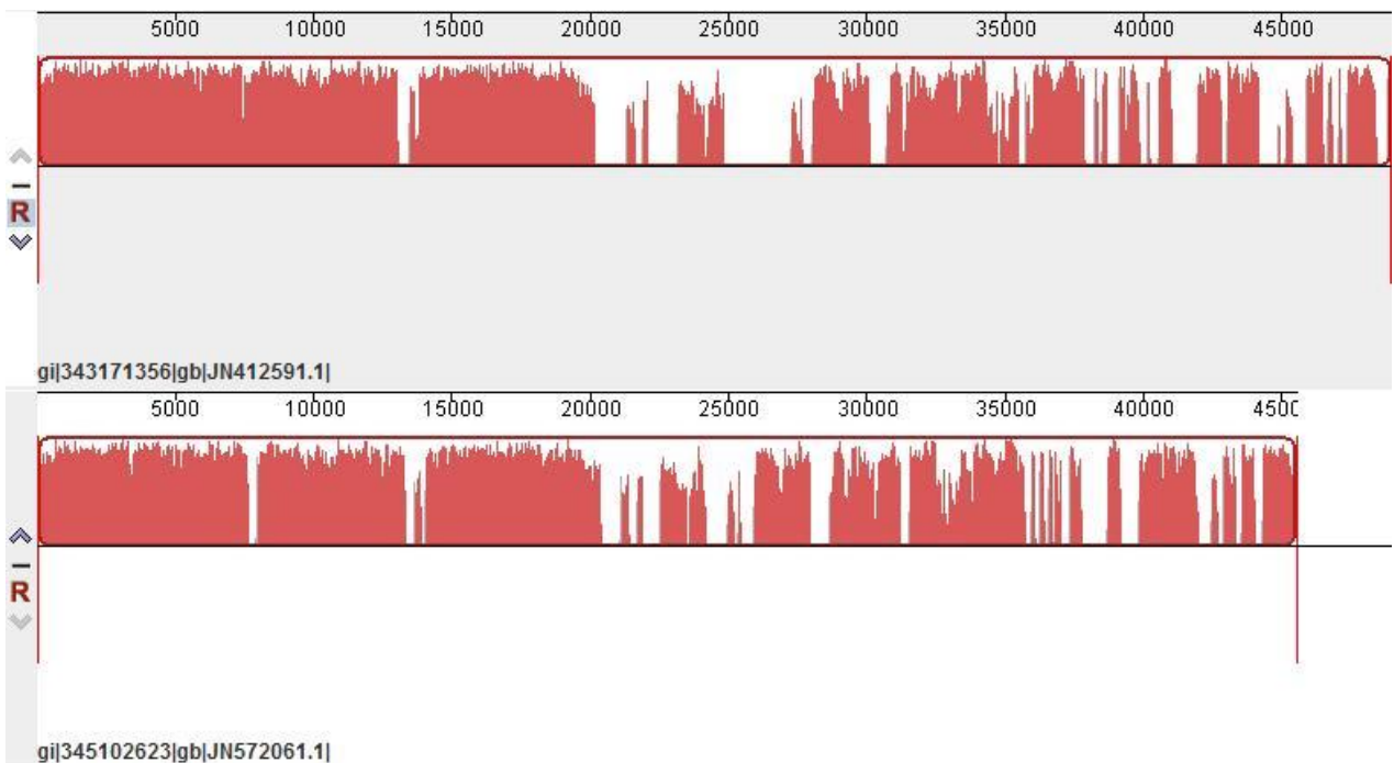
Figure 4: progressiveMauve alignment of the phage genomes belonging to the proposed genus (Bignuz top and Jebeks bottom) [5]. Colored blocks indicate the regions of 1 to 1 best alignment with rearrangement breakpoints in a different random color. The degree of sequence similarity between regions is given by a similarity plot within the colored blocks with the height of the plot proportional to the average nucleotide identity.
